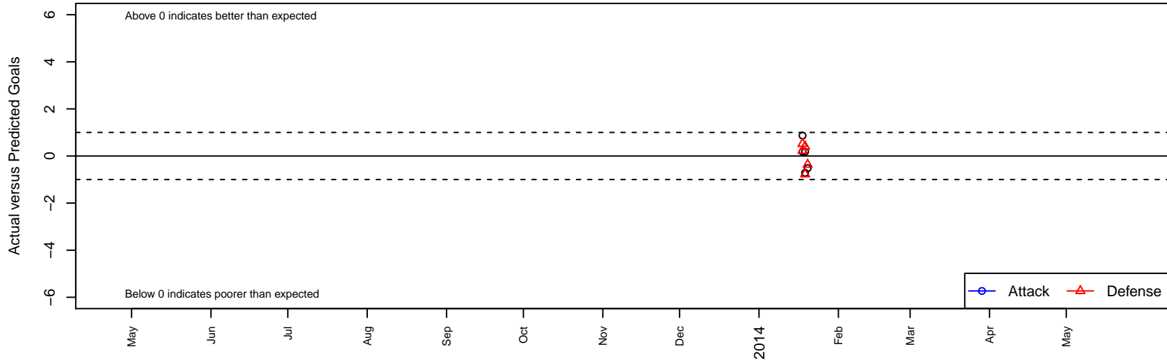
Downey FC City G01 Dots are actual minus expected GF (blue circles) and GA (red triangles). Blue line is smoothed change in attack strength. Red is smoothed change in defense strength.
